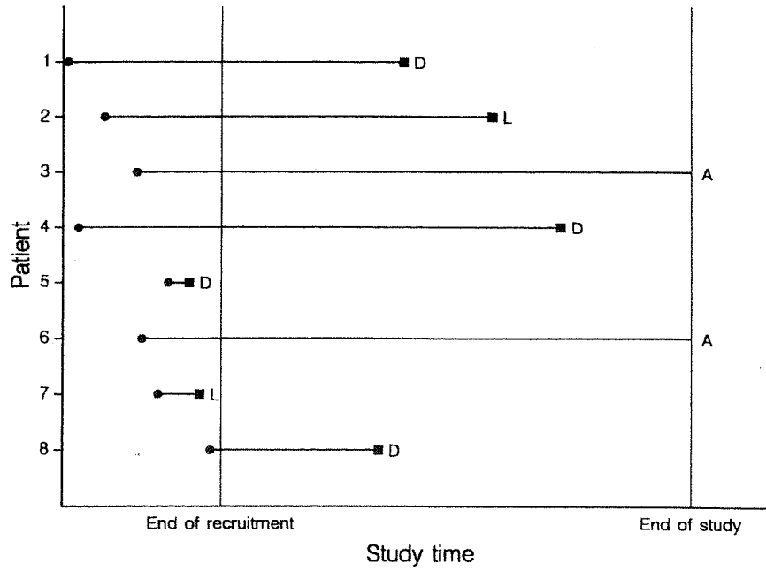
Figure 1.1 Study time for eight patients in a survival study.
