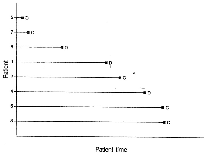
Figure 1.2 Patient time for eight patients in a survival study.
